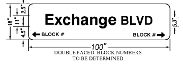
D3-1 #2 SPANWIRE MOUNTED LED SIGN
