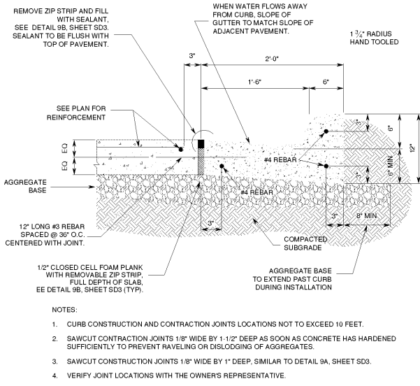
1 CATCH CURB DETAIL @ CONCRETE SLAB SD6 NTS
