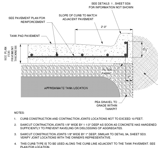
2 TANK AREA CURB DETAIL SD6 NTS
