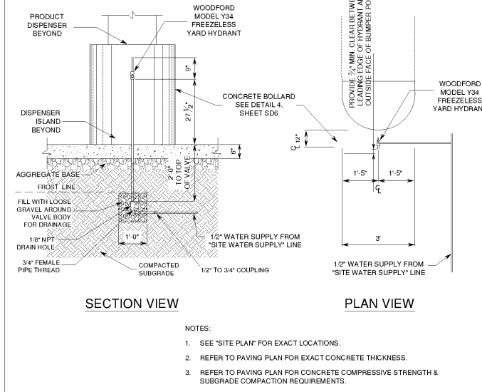
7 YARD HYDRANT DETAIL SD6 NTS
