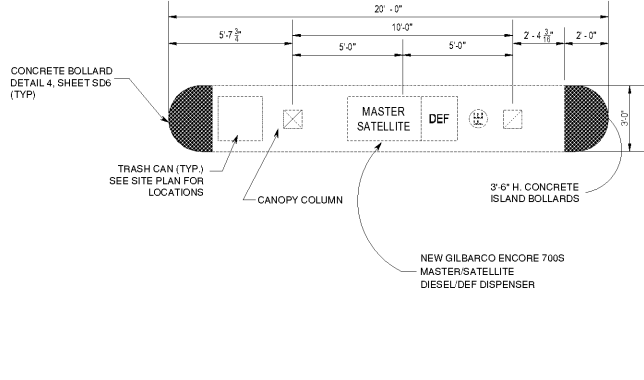
5 EDO DISPENSER ISLAND DETAIL SD6 NTS
