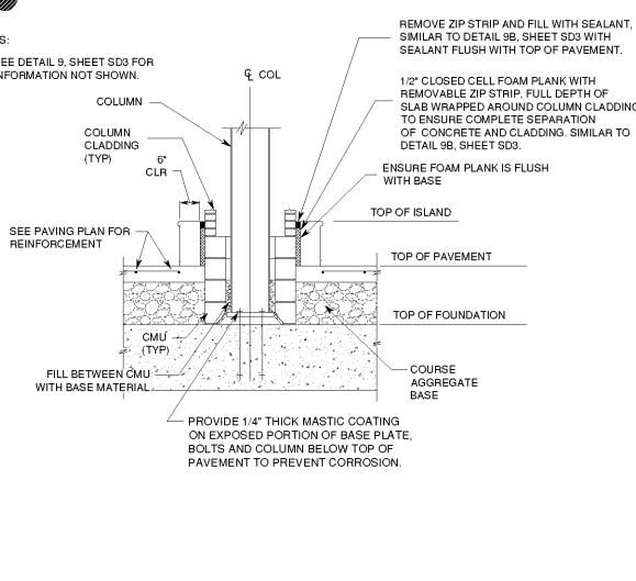
9 CANOPY COLUMN SECTION WITH COLUMN CLADDING SD6 NTS
