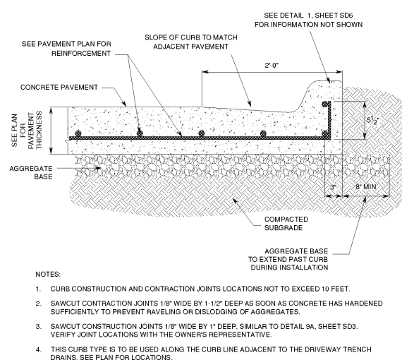
3 MONOLITHIC CURB DETAIL SD6 NTS
