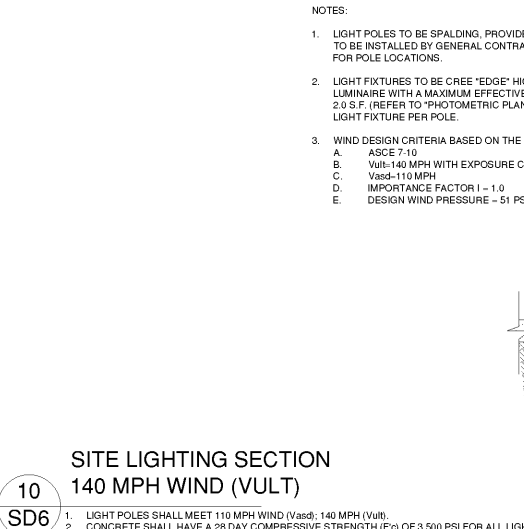
10 SITE LIGHTING SECTION 140 MPH WIND (VULT) SD6 NTS
