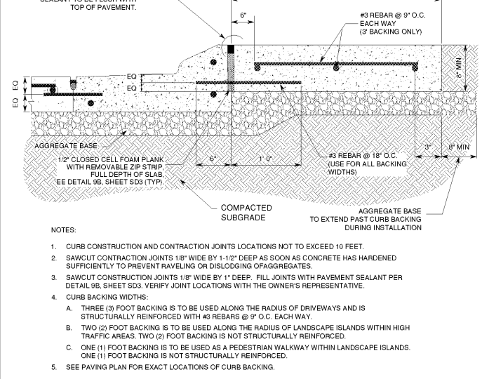
5 CONCRETE BACKING FOR ON-SITE CURB SD1 NTS
