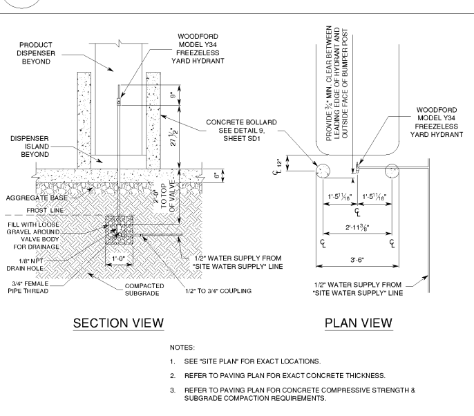
12 YARD HYDRANT DETAIL SD1 NTS
