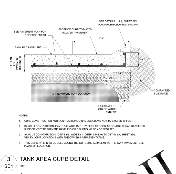
3 TANK AREA CURB DETAIL SD1 NTS
