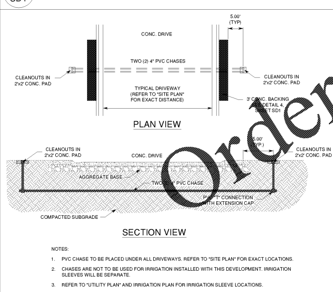
9 PVC CHASE DETAIL SD1 NTS
