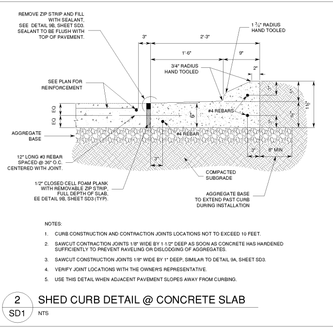
2 SHED CURB DETAIL @ CONCRETE SLAB SD1 NTS
