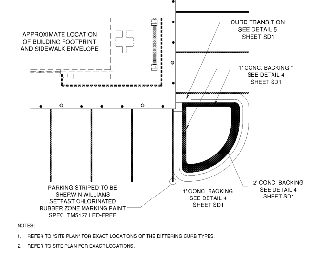
8 CONCRETE BACKING PLAN VIEW SD1 NTS
