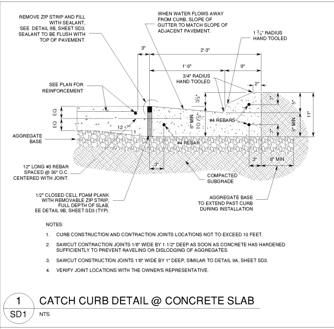
1 CATCH CURB DETAIL @ CONCRETE SLAB SD1 NTS
