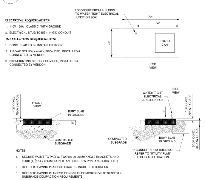
11 AIR/VAC SERVICE DETAIL SD1 NTS
