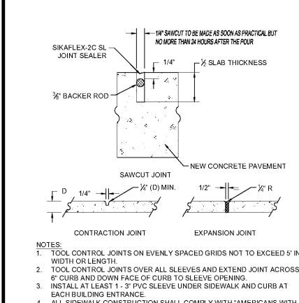
10 SIDEWALK CONTROL JOINTS
