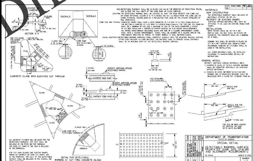
6 SPECIAL DETAIL - A4 - DETECTABLE WARNING SURFACE TRUNCATED DOME
