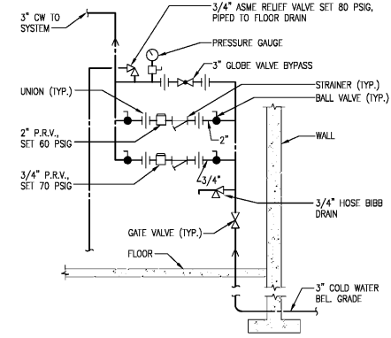
1 PRESSURE REDUCING STATION SCALE: NONE
