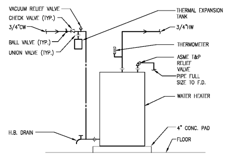
3 ELECTRIC WATER HEATER PIPING SCALE: NONE
