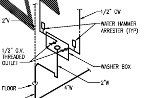
5 WASHER BOX PIPING SCALE: NONE
