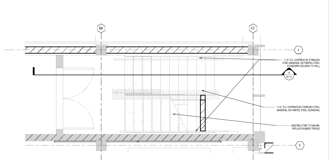
2 ENLARGED FLOOR PLAN - STAIR 1122 A7.13 SCALE: 1/2" = 1'-0"
