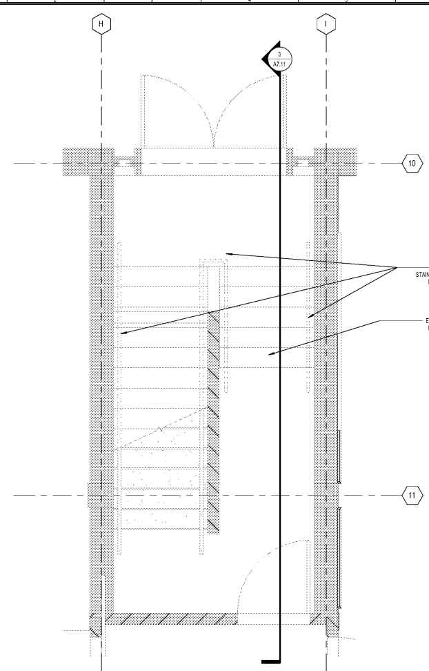
4 ENLARGED FLOOR PLAN - STAIR 2105 SCALE: 1/2" = 1'-0"
