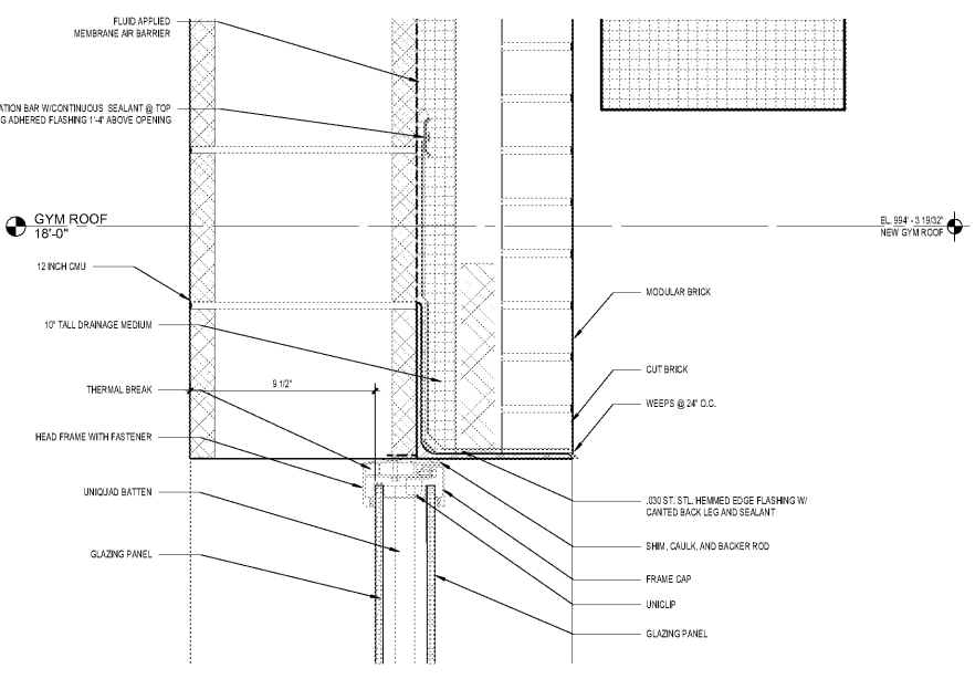
7 SECTION DTL - POLYCARB HEAD DTL SCALE: 3" = 1'-0"
