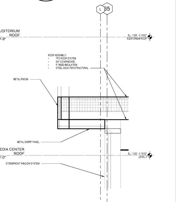
1 SECTION DTL - MEDIA CLERESTORY HEAD DTL SCALE: 1 1/2" = 1'-0"
