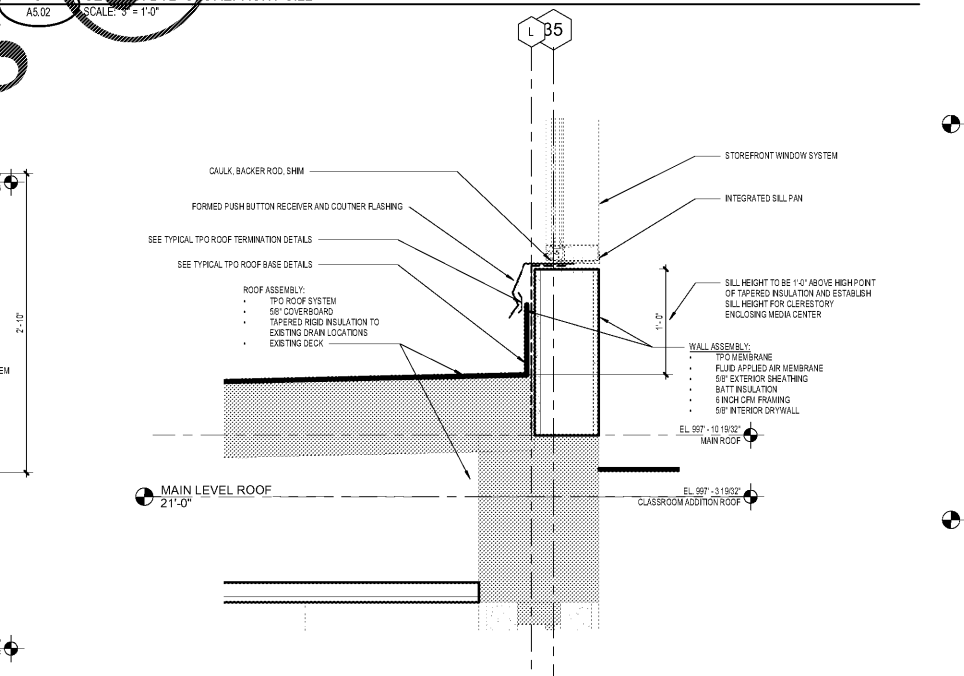
2 SECTION DTL - MEDIA CLERESTORY SILL SCALE: 1 1/2" = 1'-0"
