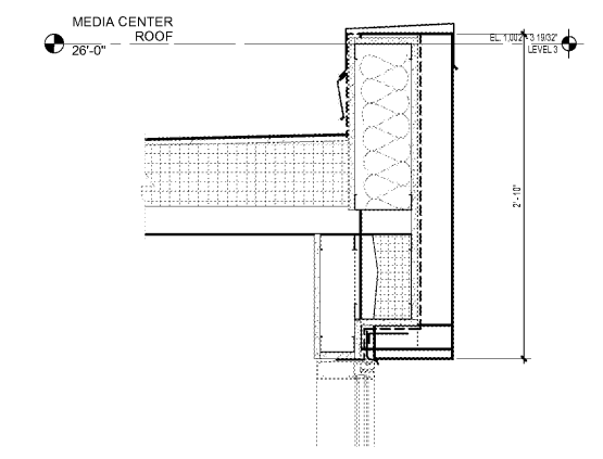
2 A5.01 ENTRY VESTIBULE - STOREFRONT HEAD DETAIL TYP. SCALE: 1 1/2" = 1'-0"
