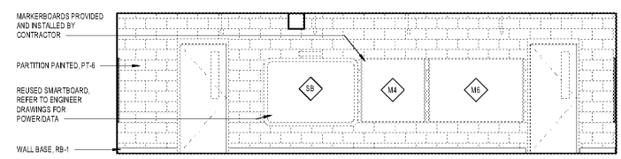
3 ELEVATION - MAKER SPACE B A4.26 SCALE: 1/4" = 1'-0"
