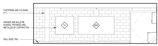
4 ELEVATION - MAKER SPACE C A4.26 SCALE: 1/4" = 1'-0"
