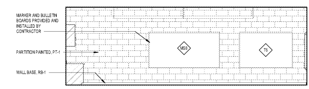
2 ELEVATION - MAKER SPACE A A4.26 SCALE: 1/4" = 1'-0"
