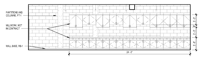
5 ELEVATION - MAKER SPACE D A4.26 SCALE: 1/4" = 1'-0"
