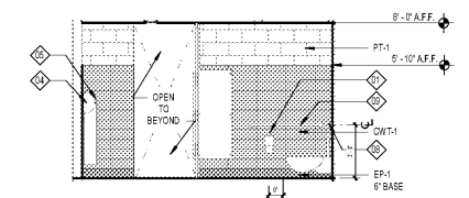
4 RR ELEVATION @ AREA A RR A4.23 SCALE: 1/4" = 1'-0"
