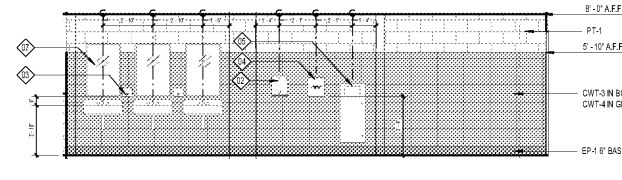
3 RR ELEVATION @ AREA A RR A4.23 SCALE: 1/4" = 1'-0"
