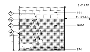
13 RR ELEVATION @ RESTROOM A4.23 SCALE: 1/4" = 1'-0"
