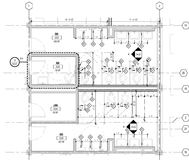
1 2ND FLOOR - AREA A - CLASSROOM RESTROOM A4.23 SCALE: 1/4" = 1'-0"
