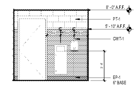
15 RR ELEVATION @ RESTROOM A4.23 SCALE: 1/4" = 1'-0"
