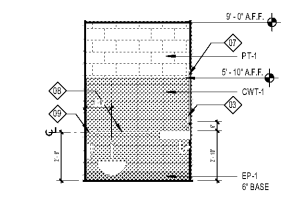
8 RR ELEVATION @ RESTROOM A4.23 SCALE: 1/4" = 1'-0"
