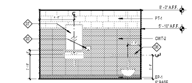
14 RR ELEVATION @ RESTROOM A4.23 SCALE: 1/4" = 1'-0"
