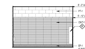
12 RR ELEVATION @ RESTROOM A4.23 SCALE: 1/4" = 1'-0"
