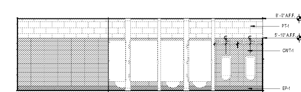
5 RR ELEVATION @ AREA A RR A4.23 SCALE: 1/4" = 1'-0"
