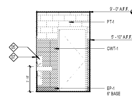
10 RR ELEVATION @ RESTROOM A4.23 SCALE: 1/4" = 1'-0"
