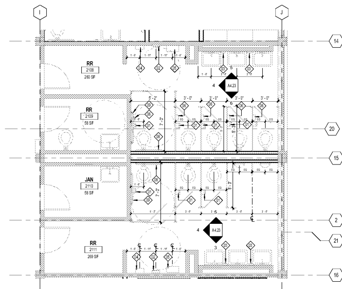
2 1ST FLOOR - AREA A - CLASSROOM RESTROOM A4.23 SCALE: 1/4" = 1'-0"
