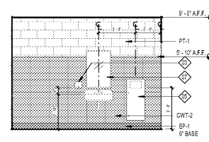
7 RR ELEVATION @ RESTROOM A4.23 SCALE: 1/4" = 1'-0"
