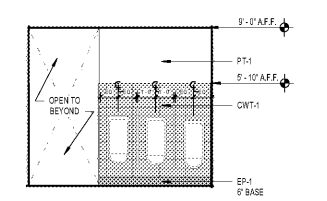
3 RR ELEVATION @ AREA B RR A4.22 SCALE: 1/4" = 1'-0"
