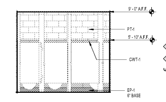
5 RR ELEVATION @ AREA B RR A4.22 SCALE: 1/4" = 1'-0"
