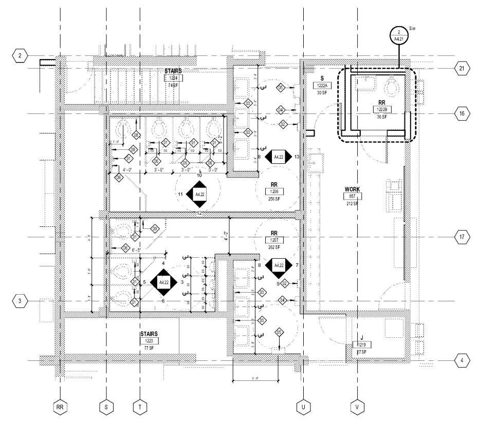
1 2ND FLOOR - AREA B - CLASSROOM RESTROOMS A4.22 SCALE: 1/4" = 1'-0"
