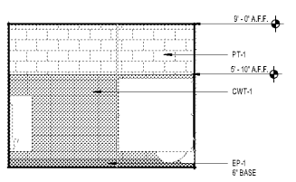
6 RR ELEVATION @ AREA B RR A4.22 SCALE: 1/4" = 1'-0"
