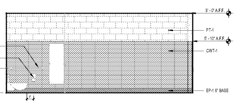
4 RR ELEVATION @ AREA B RR A4.22 SCALE: 1/4" = 1'-0"
