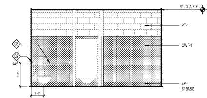
17 RR ELEVATION @ CORRIDOR RR A4.21 SCALE: 1/4" = 1'-0"
