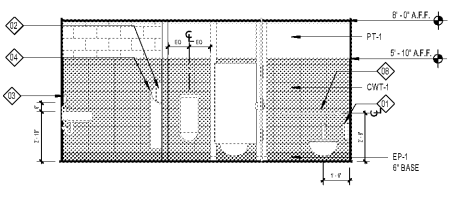
6 RR ELEVATION @ AUDITORIUM RR A4.21 SCALE: 1/4" = 1'-0"
