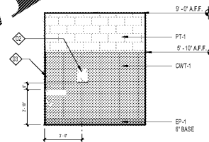
11 RR ELEVATION @ UNISEX RR A4.21 SCALE: 1/4" = 1'-0"
