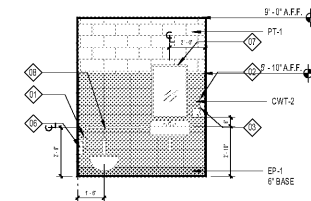
10 RR ELEVATION @ UNISEX RR A4.21 SCALE: 1/4" = 1'-0"
