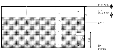
4 RR ELEVATION @ AUDITORIUM RR A4.21 SCALE: 1/4" = 1'-0"
