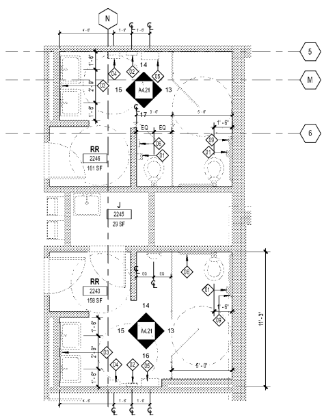
12 2ND FLOOR PLAN - AREA B - CORRIDOR RESTROOM A4.21 SCALE: 1/4" = 1'-0"
