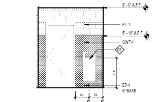
8 RR ELEVATION @ UNISEX RR A4.21 SCALE: 1/4" = 1'-0"
