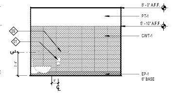
7 RR ELEVATION @ AUDITORIUM RR A4.21 SCALE: 1/4" = 1'-0"
