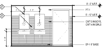
5 RR ELEVATION @ AUDITORIUM RR A4.21 SCALE: 1/4" = 1'-0"
