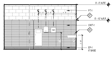
16 RR ELEVATION @ CORRIDOR RR A4.21 SCALE: 1/4" = 1'-0"
