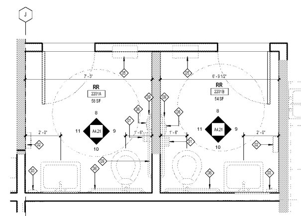
3 2ND FLOOR - AREA A - NURSE RESTROOM A4.21 SCALE: 1/2" = 1'-0"
