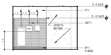
19 RR ELEVATION @ AUDITORIUM RR A4.21 SCALE: 1/4" = 1'-0"
