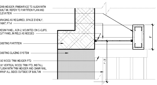
5 SECTION - MEDIA CTR GWB HEADER SCALE: 1 1/2" = 1'-0"
