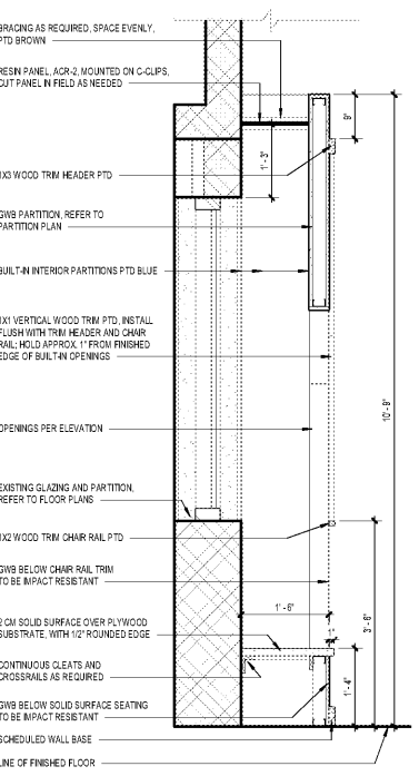
4 SECTION - MEDIA CTR BUILT-IN SCALE: 3/4" = 1'-0"
