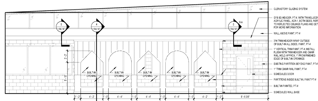
3 ELEVATION - MEDIA CENTER - PLAN EAST SCALE: 1/4" = 1'-0"
