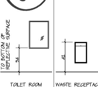
TOILET ROOM MIRROR
