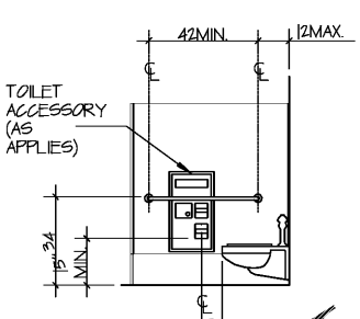
2/D - SIDE ELEVATION
