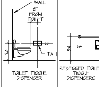
TOILET TISSUE DISPENSER
