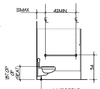
2/B - SIDE ELEVATION
