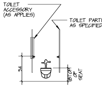
2/A - FIXTURE ELEVATION
