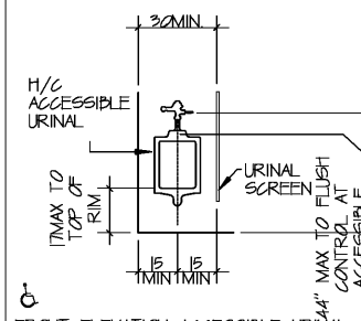
FRONT ELEVATION ACCESSIBLE URINAL STALL
