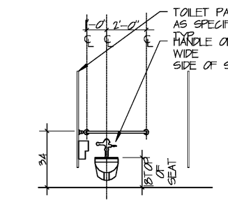
3/A - FIXTURE ELEVATION
