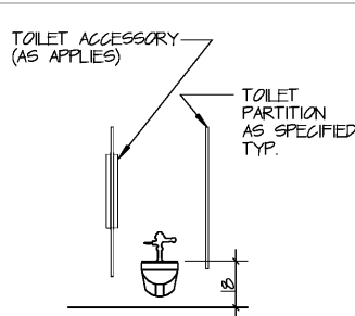
1/A - FIXTURE ELEVATION
