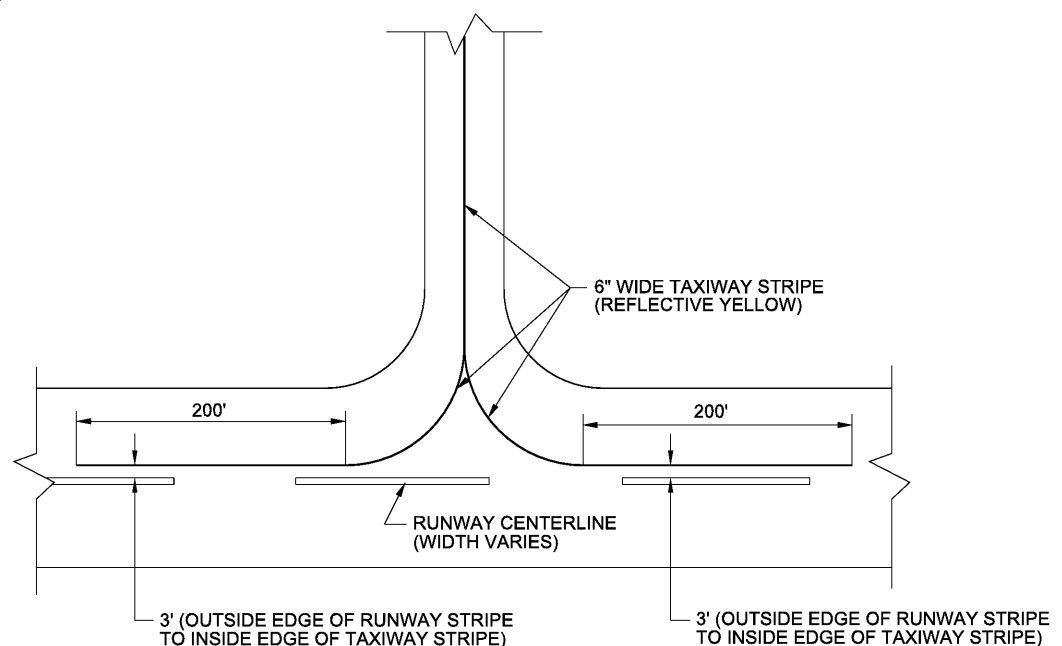
TAXIWAY CENTERLINE MARKING NOT TO SCALE
