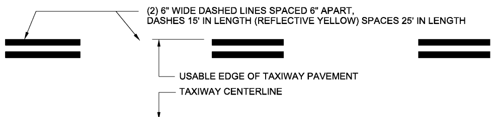
TAXIWAY EDGE APRON MARKING NOT TO SCALE
