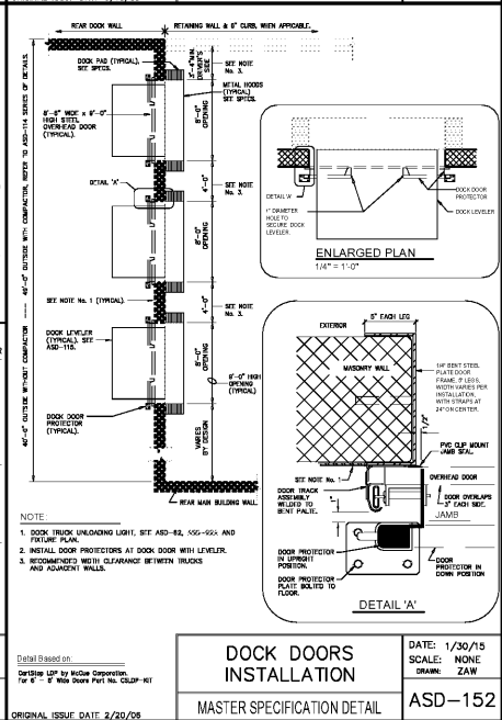
DOCK DOORS INSTALLATION MASTER SPECIFICATION DETAIL ASD-152 DATE: 1/30/15 SCALE: NONE DRAWN: ZAW
