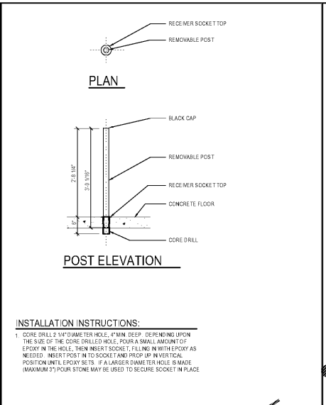
WALL TO FLOOR BASE TYPE-D MASTER SPECIFICATION DETAIL ASD-51D DATE: 11/7/13 SCALE: NONE DRAWN: ZAW
