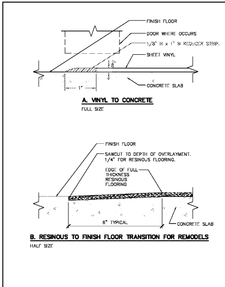
A. VINYL TO CONCRETE FULL SIZE
