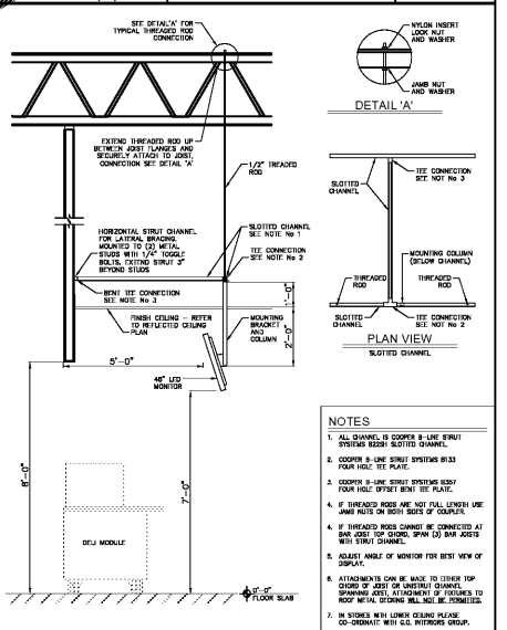
SUPPORT FOR CONDENSER WITH LEGS - EXISTING CONST. MASTER SPECIFICATION DETAIL ASD-82 DATE: 3/2/15 SCALE: NONE DRAWN: ZAW
