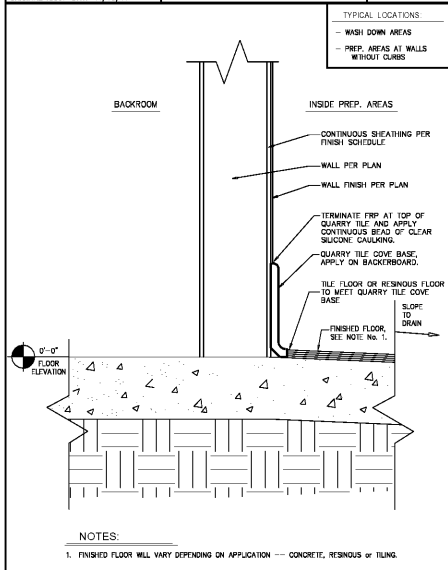
B. RESINOUS TO FINISH FLOOR TRANSITION FOR REMODELS HALF SIZE
