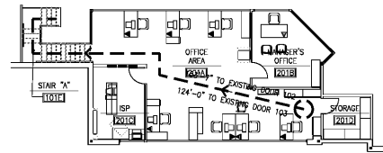
2 MEZZANINE EGRESS PLAN GO.2 3/32" = 1'-0"
