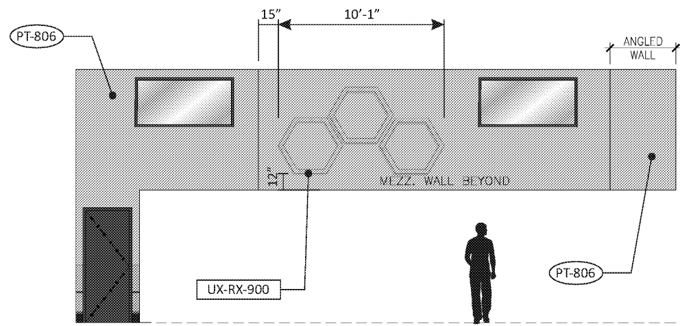
E - INTERIOR ELEVATION
