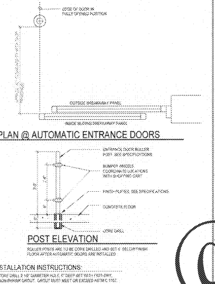
ENTRANCE DOOR ROLLER POST INSTALLATION MASTER SPECIFICATION DETAIL ASD-20
