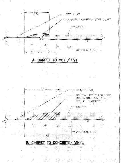
A. CARPET TO VCT / LVT FULL SIZE
