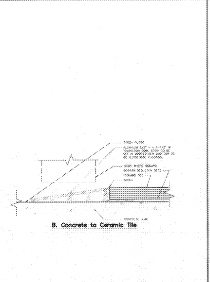
B. Concrete to Ceramic Tile HALF SIZE
