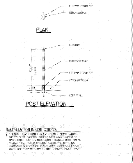
REMOVABLE PROTECTIVE POST INSTALLATION MASTER SPECIFICATION DETAIL ASD-19
