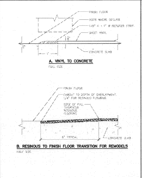
A. VINYL TO CONCRETE FULL SIZE
