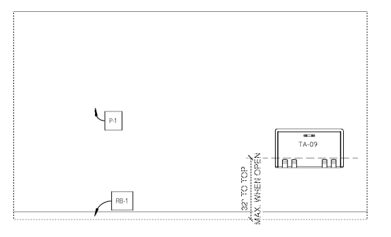
9 RESTROOMS - ELEV C 3/8" = 1'-0"
