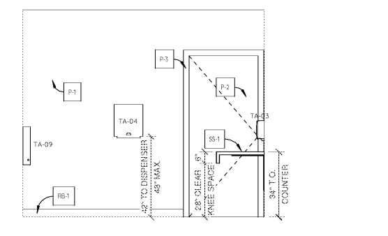
8 RESTROOMS - ELEV B 3/8" = 1'-0"
