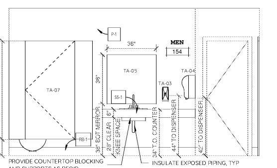
10 RESTROOM - ELEV D 3/8" = 1'-0"
