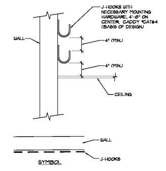
3 J-HOOK DETAIL NOT TO SCALE
