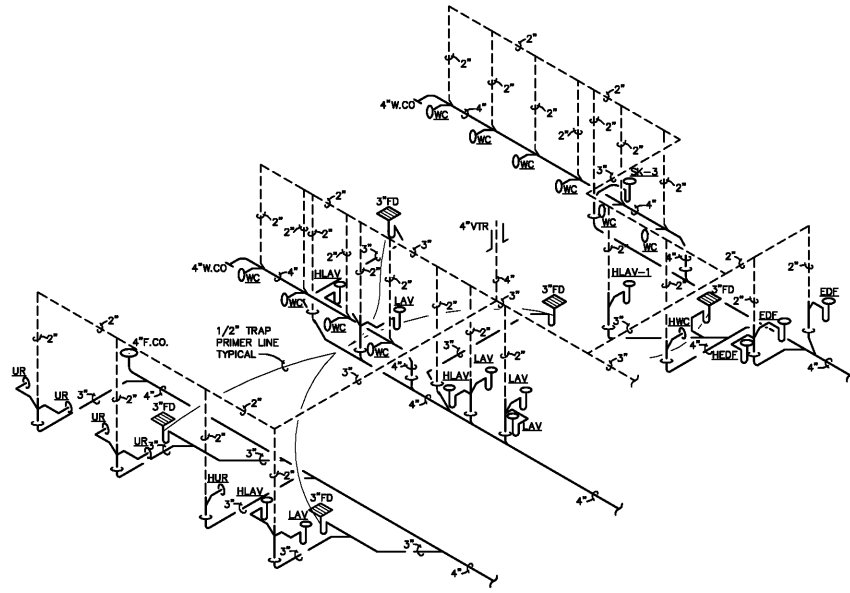
2 PLUMBING - RISER DIAGRAM P2.1 NO SCALE
