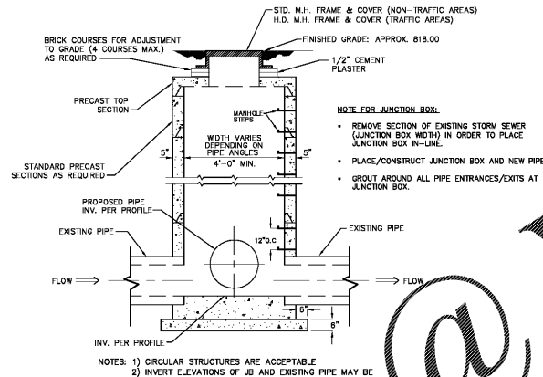
DOGHOUSE MANHOLE DETAIL (NOT TO SCALE)
