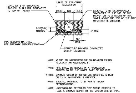
STORM SEWER TRENCHING & BACKFILLING (NOT TO SCALE)
