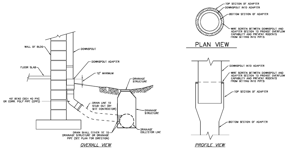
DOWNSPOUT COLLECTOR ADAPTER DETAIL (NOT TO SCALE)
