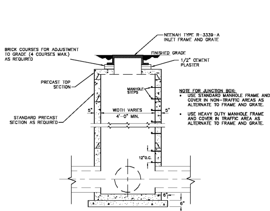
PRECAST DROP INLET & JUNCTION BOX DETAIL (NOT TO SCALE)
