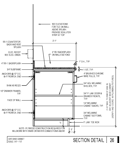
SECTION 26
