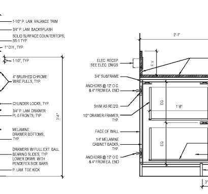
SECTION 04
