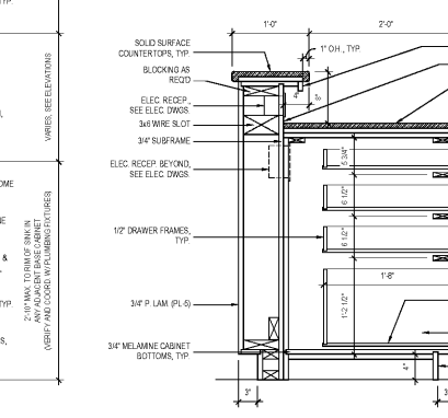
SECTION 05
