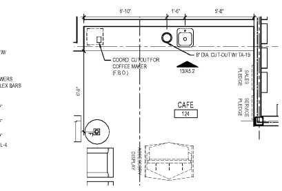
ENLARGED PLAN 24
