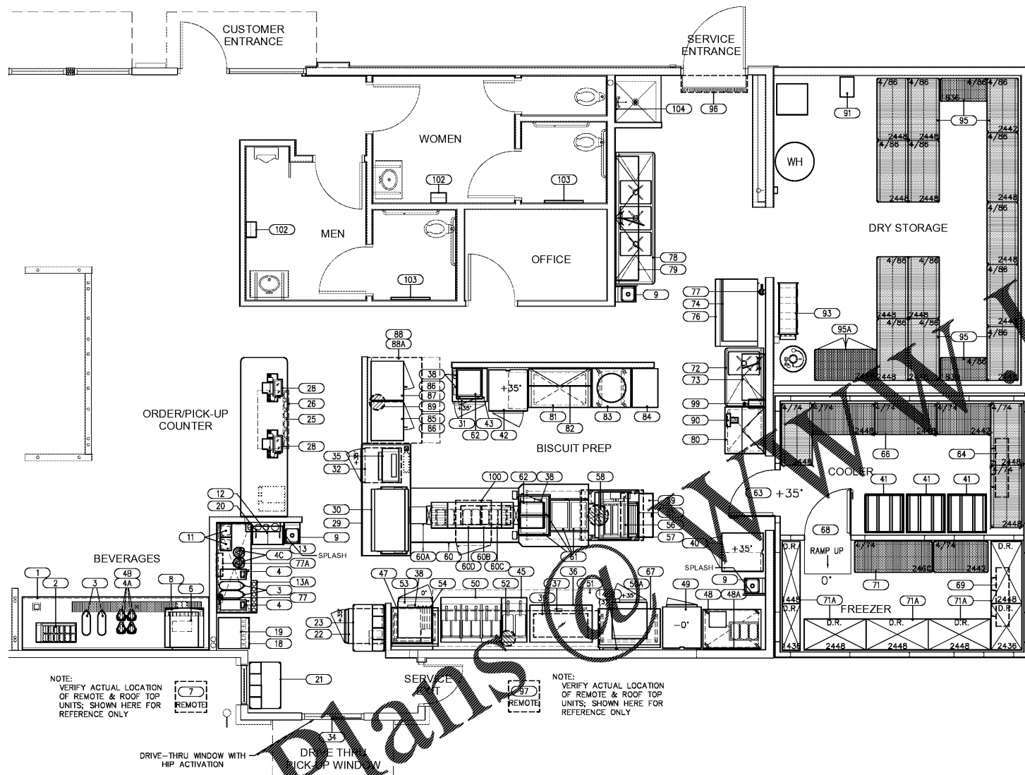
FOODSERVICE EQUIPMENT PLAN SCALE: 1/4" = 1'-0"
