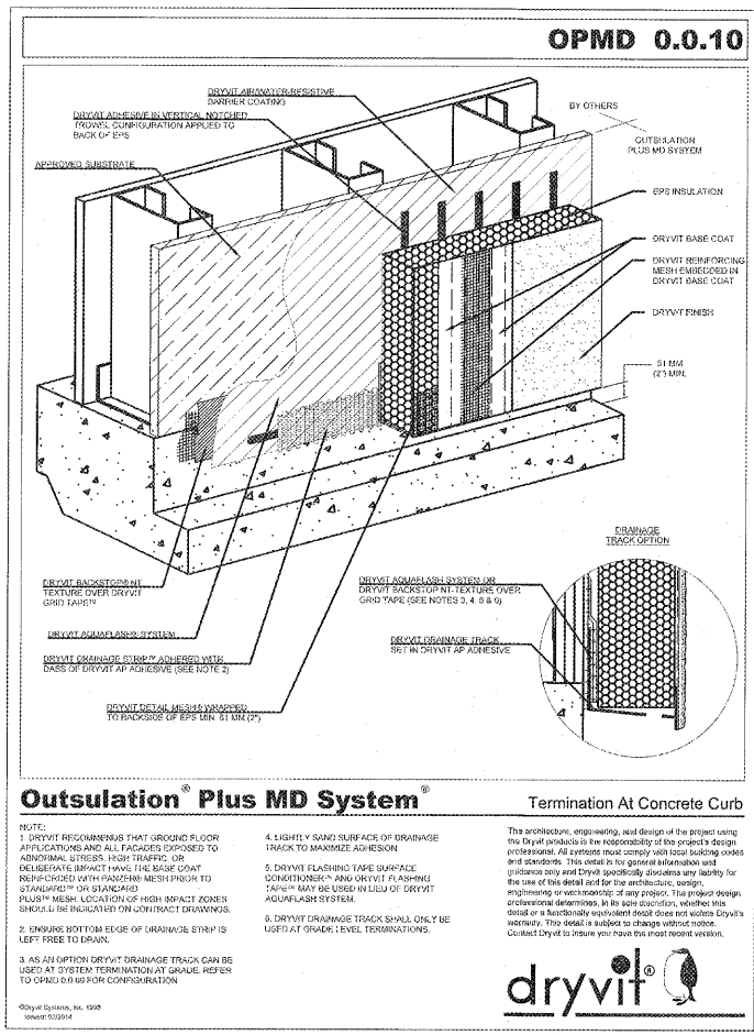
Outslulation Plus MD System Termination At Concrete Curb
