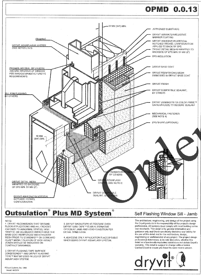
Outslulation Plus MD System Self Flashing Window Sill - Jamb
