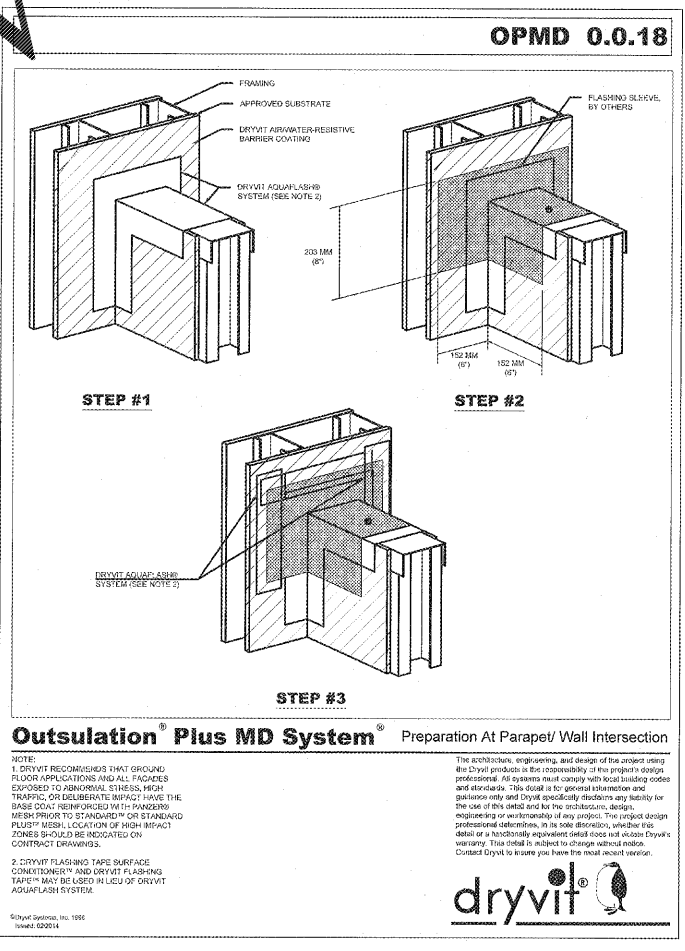
Outslulation Plus MD System Preparation At Parapet Wall Intersection
