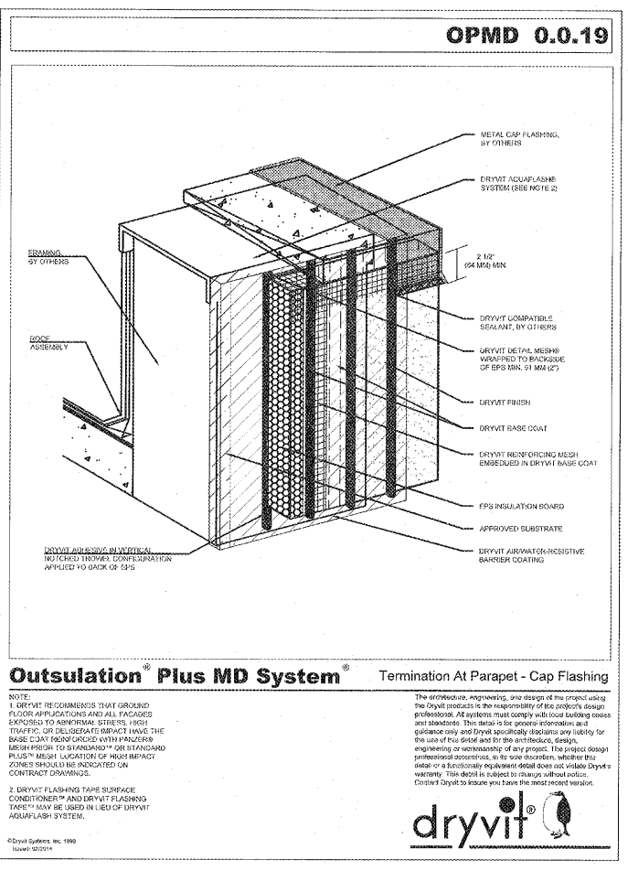
Outslulation Plus MD System Termination At Parapet - Cap Flashing
