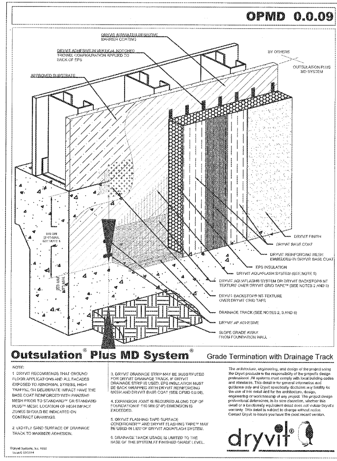
Outslulation Plus MD System Grade Termination with Drainage Track
