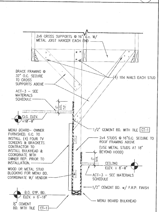
MENU BOARD BULKHEAD DTL. SCALE: 1" = 1'-0" ⑦
