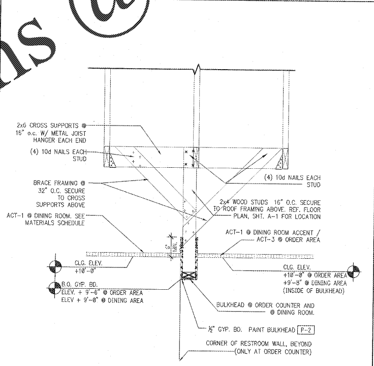
BULKHEAD DTL. • ORDER COUNTER / • DINING ROOM SCALE: 1" = 1'-0" ⑤
