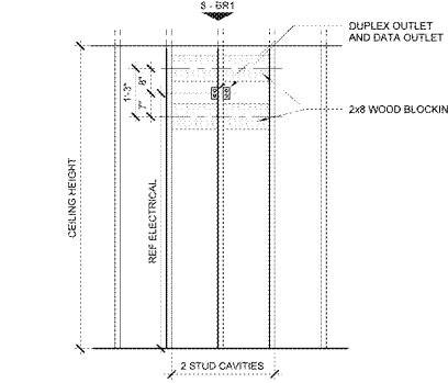
7 TV BRACKET BLOCKING 1 1/2" = 1'-0"
