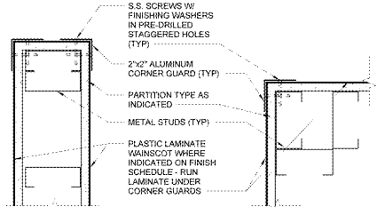
6 CORNER GUARD 3" = 1'-0"
