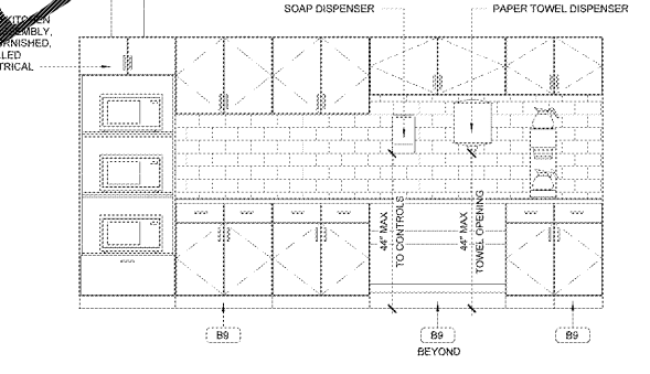
3 MODULAR CABINET ASSEMBLY ELEVATION 1 1/2" = 1'-0"
