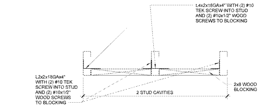
8 TV BRACKET BLOCKING PLAN 1 1/2" = 1'-0"
