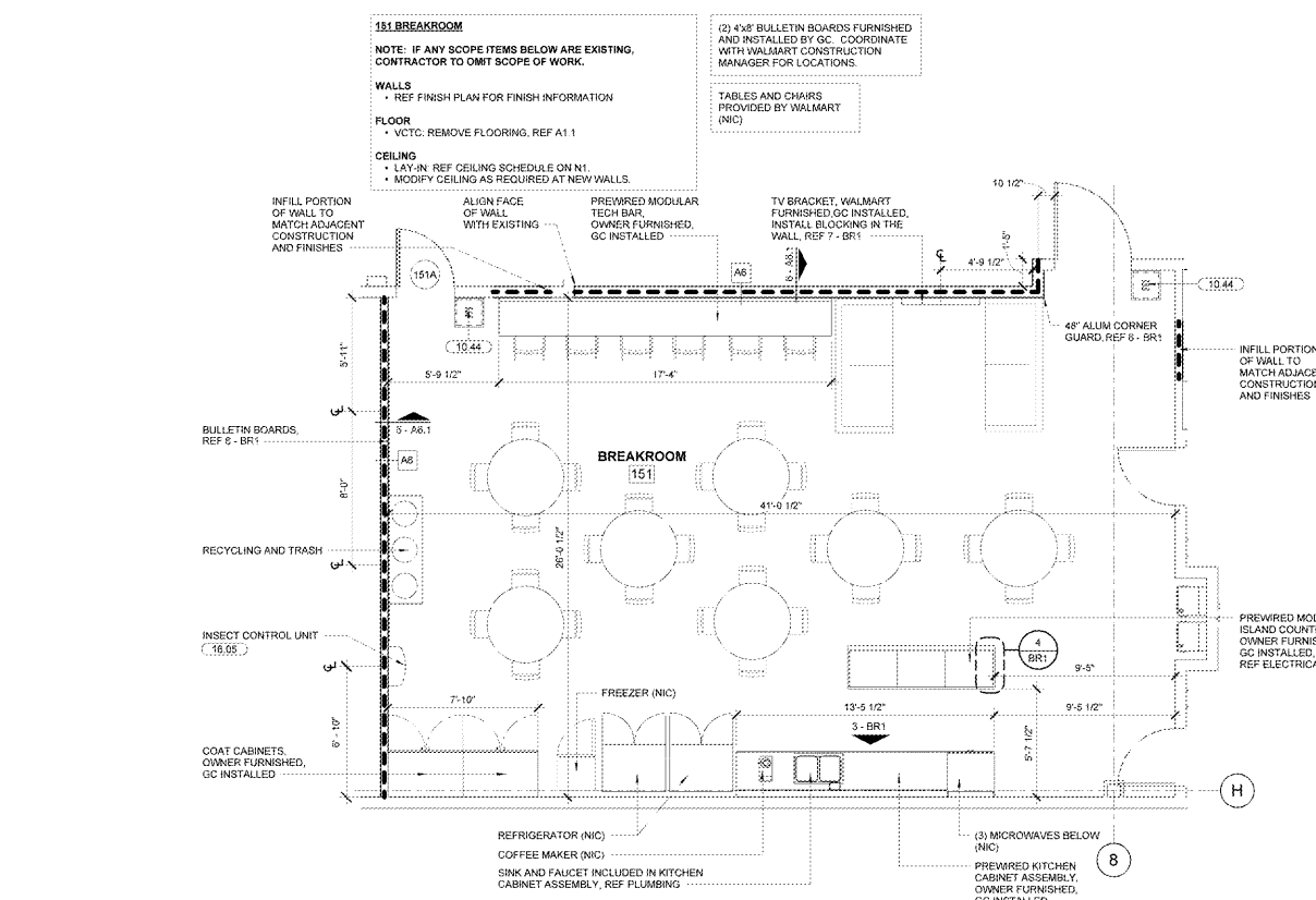
1 ENLARGED PLAN 1/4" = 1'-0"
