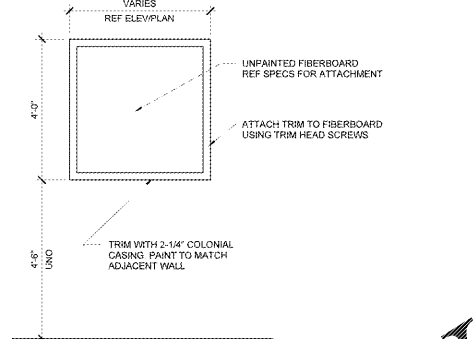
5 TACK BULLETIN BOARD 1 1/2" = 1'-0"
