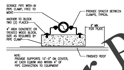
ROOF MOUNTED PIPE SUPPORT DETAIL NOT TO SCALE
