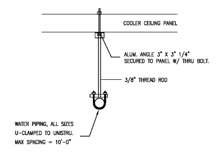
PIPE HANGING DETAIL NOT TO SCALE
