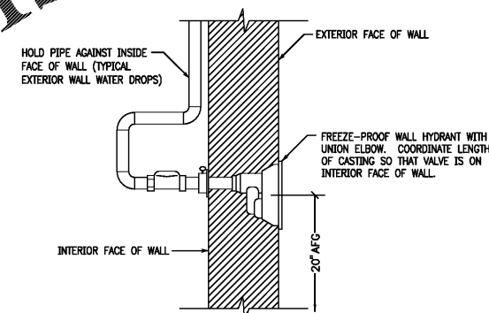
3 WALL HYDRANT DETAIL SCALE: NONE
