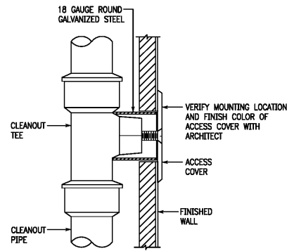
8 WALL CLEANOUT DETAIL SCALE: NONE
