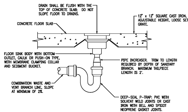
7 FLOOR SINK DETAIL SCALE: NONE
