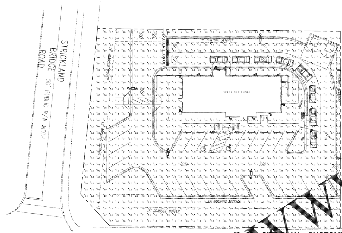
1 SITE PLAN - PHOTOMETRICS SCALE: 1" = 20'-0"
