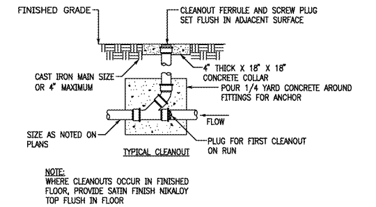
3 INTERIOR CLEANOUT DETAIL SCALE: NONE
