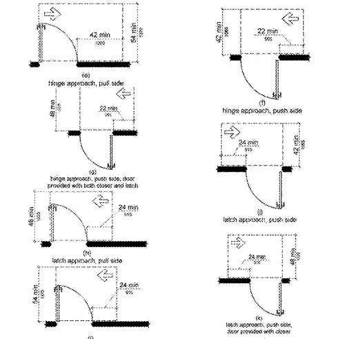
Figure 404.2.4.1 (cont.) Maneuvering Clearances of Manual Swinging Doors and Gates
