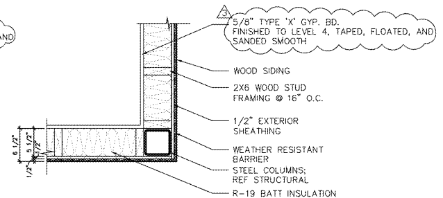
3 WALL DETAIL SCALE: 1 1/2" = 1'-0"
