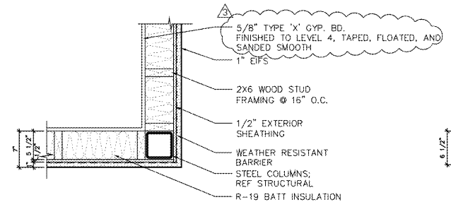
2 WALL DETAIL SCALE: 1 1/2" = 1'-0"
