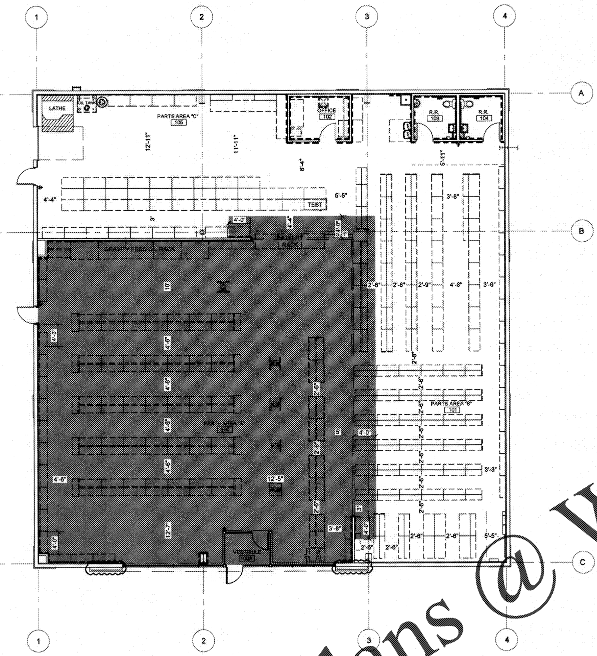
1 INTERIOR FINISH PLAN A1.2 SCALE: 1/8" = 1'-0"
