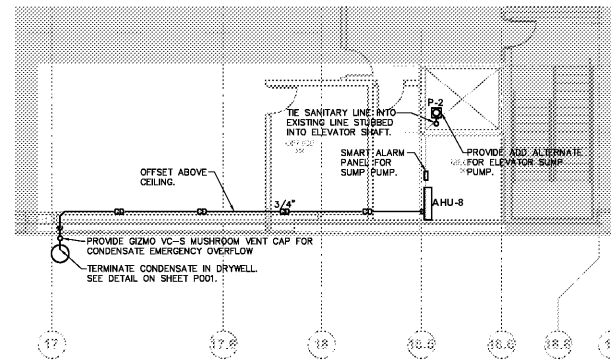
3 PARTIAL ALTERNATE FIRST LEVEL PLUMBING PLAN SCALE: 1/8" = 1'-0"
