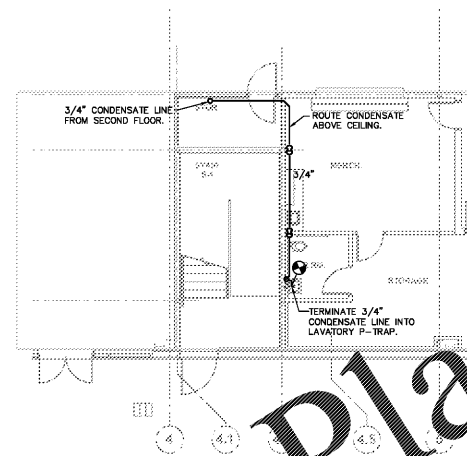
2 PARTIAL ALTERNATE FIRST LEVEL PLUMBING PLAN SCALE: 1/8" = 1'-0"
