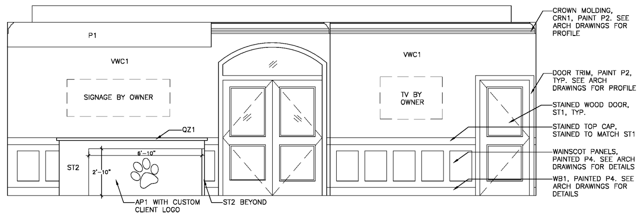
1 PUBLIC LOBBY ELEVATION - RECEPTION DESK ID-3 SCALE: 3/8" = 1'-0"
