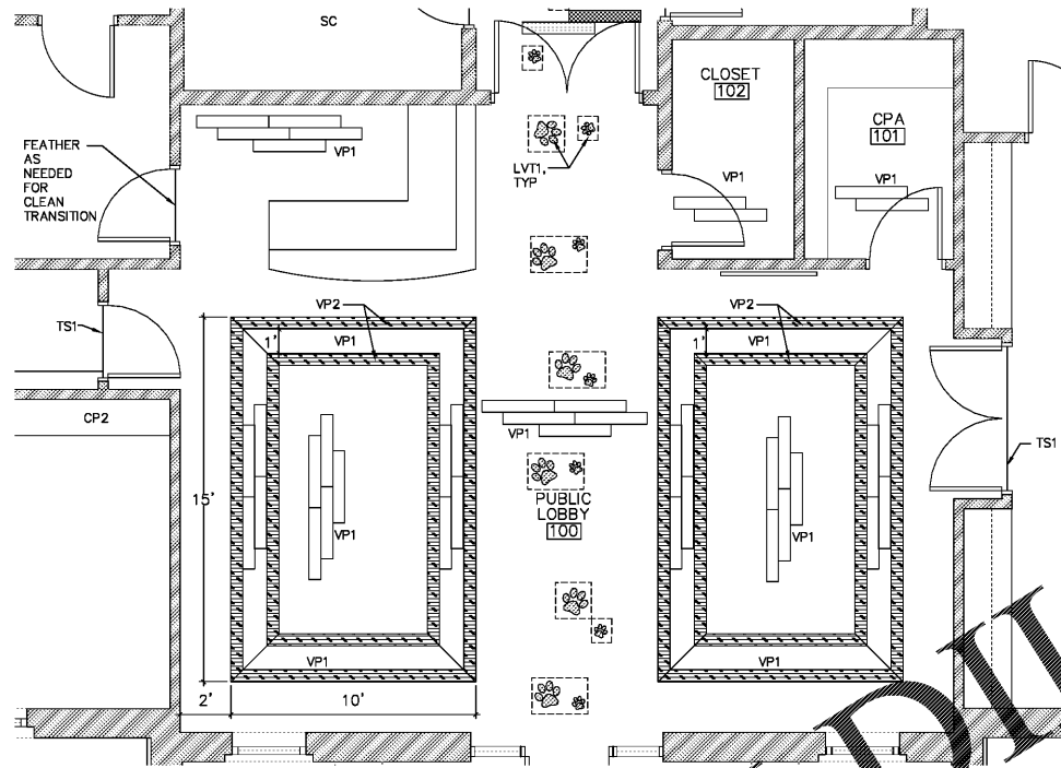
2 PUBLIC LOBBY FLOOR PATTERN DETAIL
