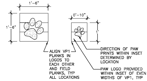
1 PAW PRINT DETAIL SCALE: 3/4" = 1'-0"
