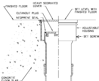
FLOOR CLEANOUT DETAIL NO SCALE
