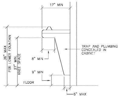
ACCESSIBLE EWC NO SCALE
