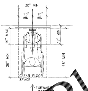
ACCESSIBLE SINK/LAV NO SCALE
