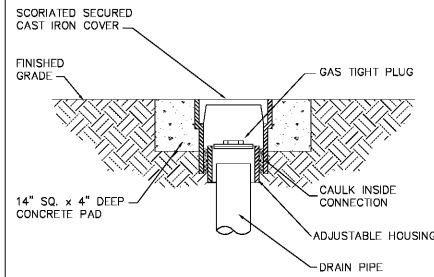
GRADE CLEANOUT NO SCALE
