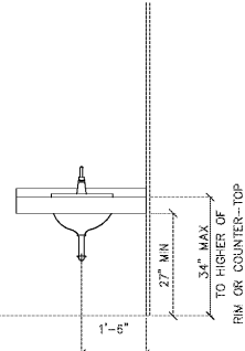
ACCESSIBLE SINK/LAV NO SCALE
