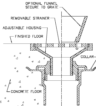
FLOOR DRAIN DETAIL NO SCALE
