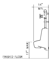
ACCESSIBLE URINAL NO SCALE
