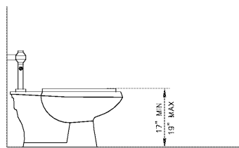
ACCESSIBLE WATERCLOSET NO SCALE
