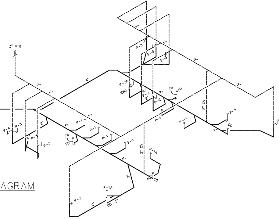
PLUMBING DETAILS NO SCALE
