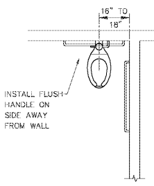
ACCESSIBLE WATERCLOSET NO SCALE
