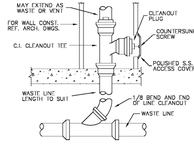
WALL CLEANOUT DETAIL NO SCALE
