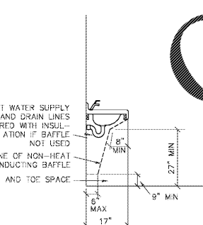
ACCESSIBLE SINK/LAV NO SCALE
