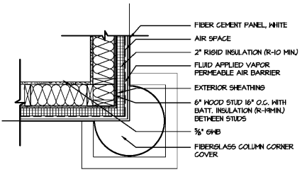
10 PLAN DETAILS A5.1 SCALE: 3/4" = 1'-0"
