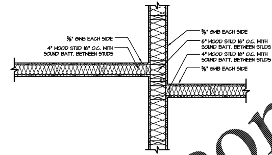
4 PLAN DETAILS A5.1 SCALE: 3/4" = 1'-0"
