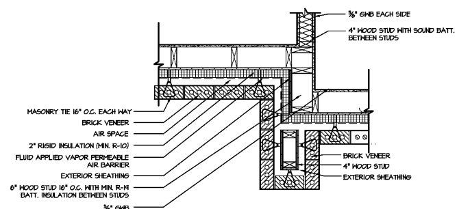
12 PLAN DETAILS A5.1 SCALE: 3/4" = 1'-0"
