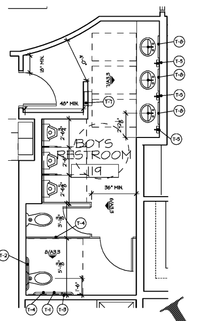
5 ENLARGED PLAN BOYS A3.3 SCALE: 1/4" = 1'-0"
