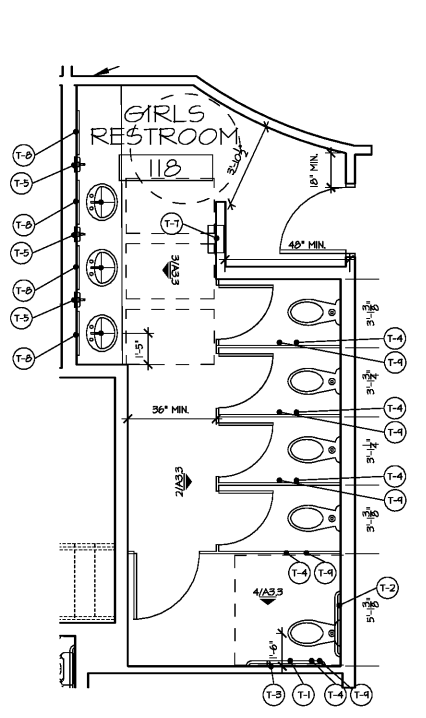
1 ENLARGED PLAN GIRLS A3.3 SCALE: 1/4" = 1'-0"
