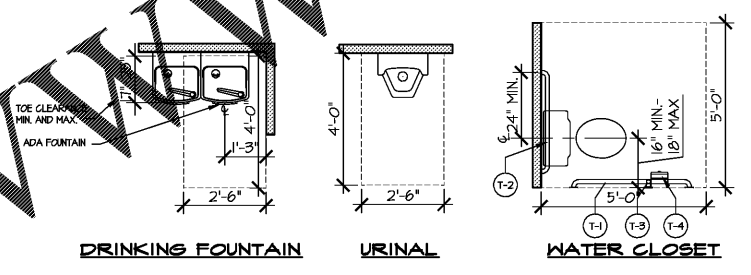
5 ENLARGED PLAN BOYS A3.3 SCALE: 1/4" = 1'-0"
