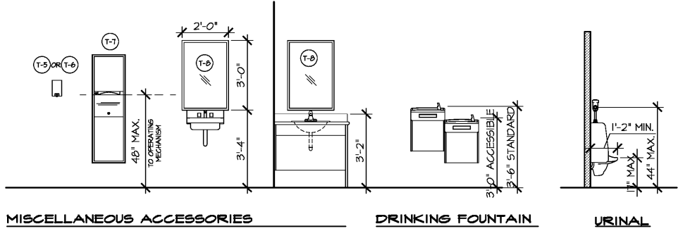
12 MOUNTING HEIGHTS A3.3 SCALE: 1/4" = 1'-0"
