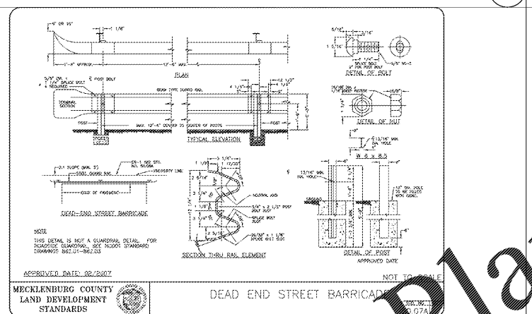
MECKLENBURG COUNTY LAND DEVELOPMENT STANDARDS DEAD END STREET BARRICADE
