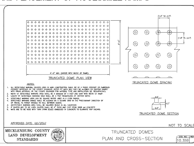
MECKLENBURG COUNTY LAND DEVELOPMENT STANDARDS TRUNCATED DOMES PLAN AND CROSS-SECTION
