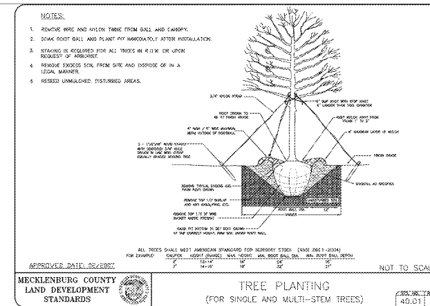
TREE PLANTING
