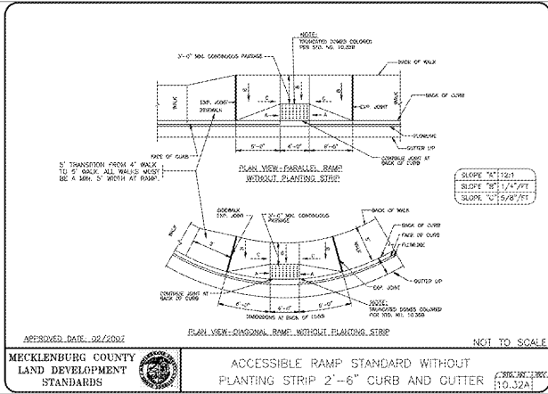
ACCESSIBLE RAMP STANDARD
