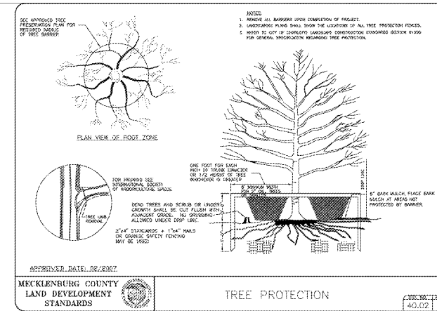
TREE PROTECTION
