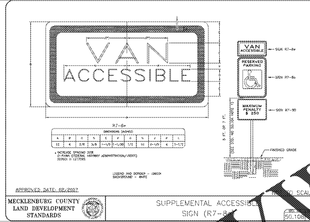
SUPPLEMENTAL ACCESSIBLE SIGN
