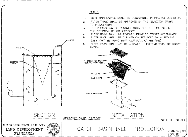
CATCH BASIN INLET PROTECTION
