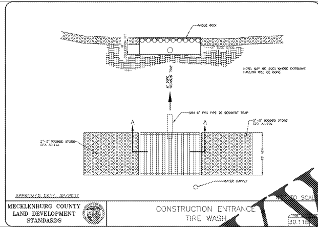
CONSTRUCTION ENTRANCE TIRE WASH
