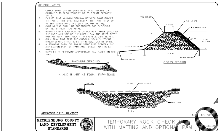
TEMPORARY ROCK CHECK DAM
