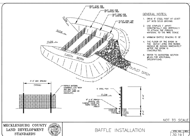
BAFFLE INSTALLATION
