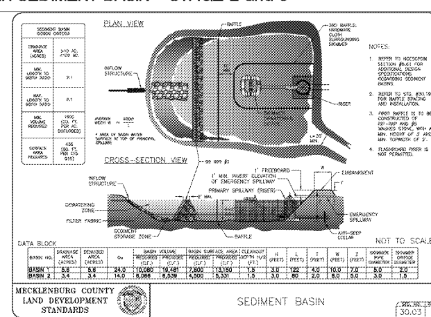
SKIMMER SEDIMENT BASIN - STAGE 1
