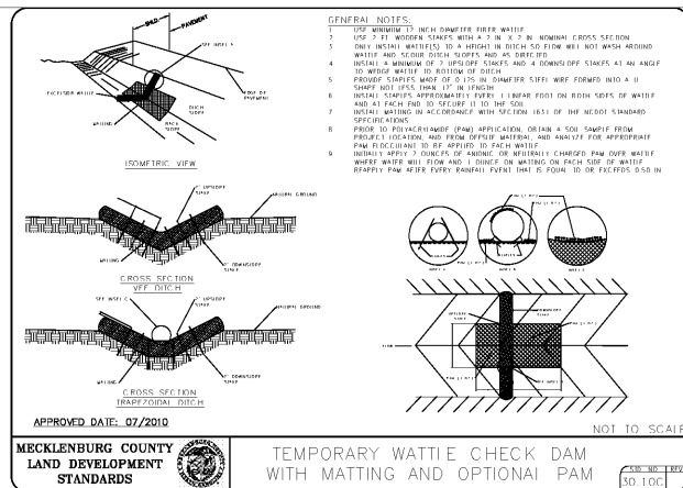
TEMPORARY WATTLE CHECK DAM
