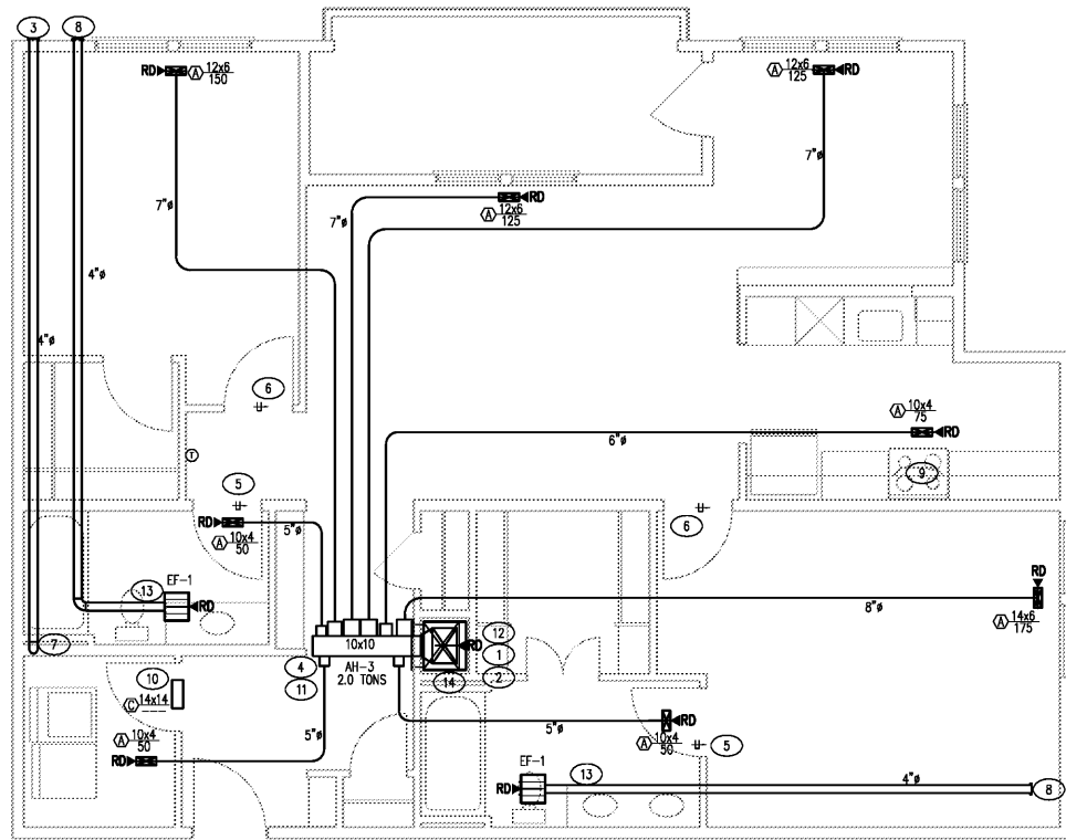
1 UNIT C2E - PLAN - MECHANICAL 1/4" = 1'-0"
