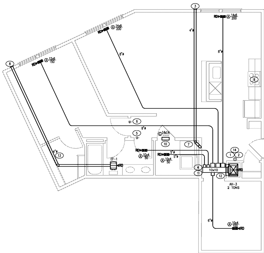
1 UNIT B6 - PLAN - MECHANICAL 1/4" = 1'-0"
