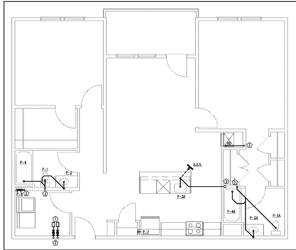
1 UNIT C3 HC PLUMBING PLAN 1/4" = 1'-0"
