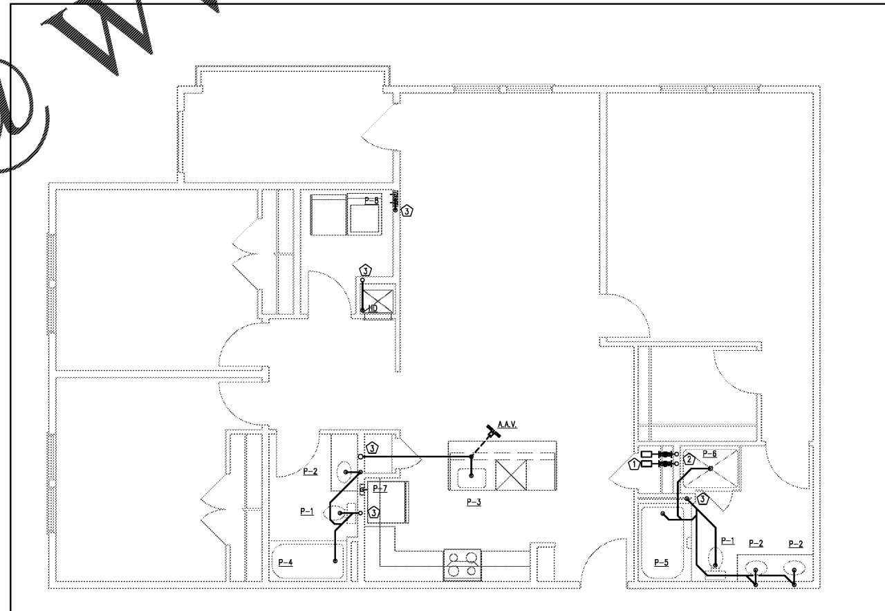
6 UNIT D1 PLUMBING PLAN 1/4" = 1'-0"
