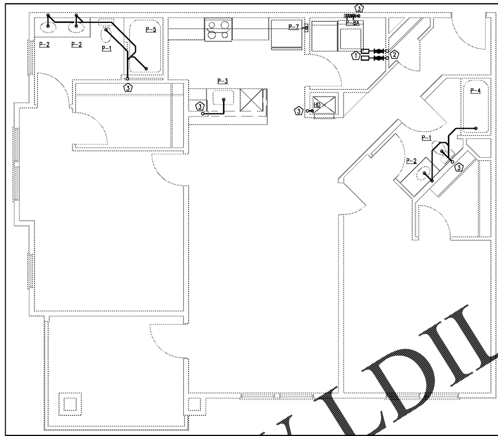
2 UNIT C5 PLUMBING PLAN 1/4" = 1'-0"
