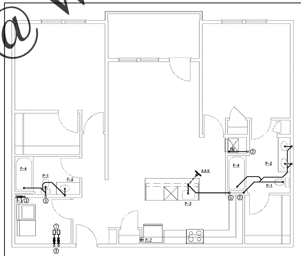
6 UNIT C3 PLUMBING PLAN 1/4" = 1'-0" (UNIT C3S & C4 SIMILAR)
