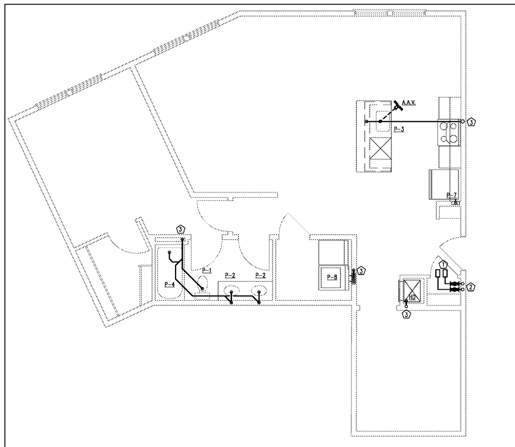
1 UNIT B6 PLUMBING PLAN 1/4" = 1'-0" (UNIT B6J SIMILAR)
