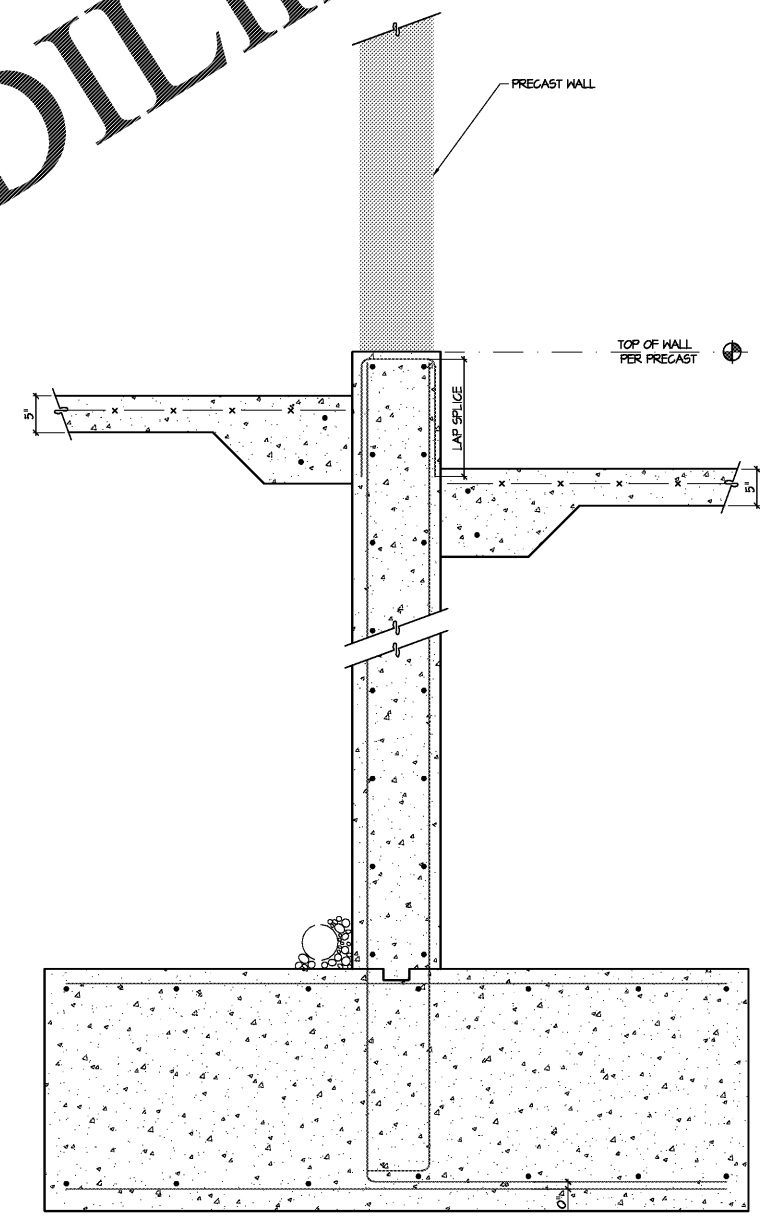
1 SECTION AT RETAINING WALL NOT TO SCALE
